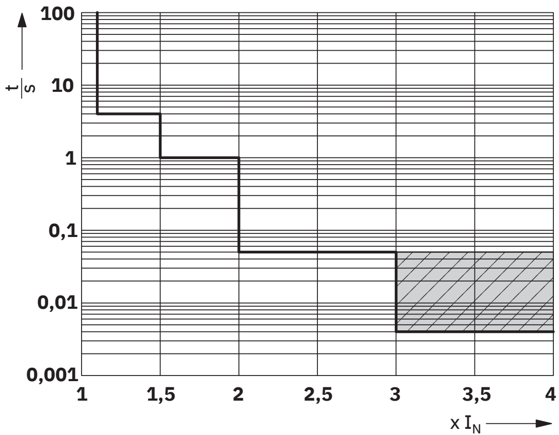
Trigger characteristic in the DC range
